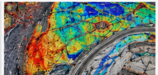
Hyperspectral Imaging
